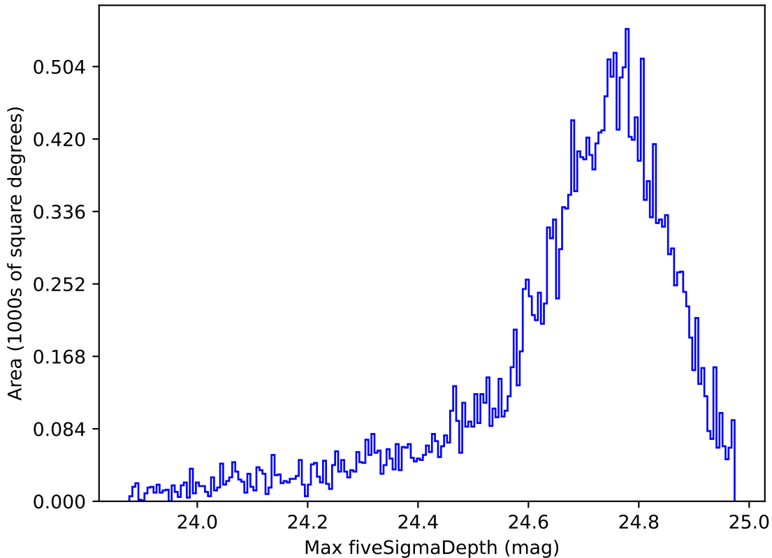
too_elab_r8_d3_gz_v3.4_10yrs All sky r band: Max fiveSigmaDepth
