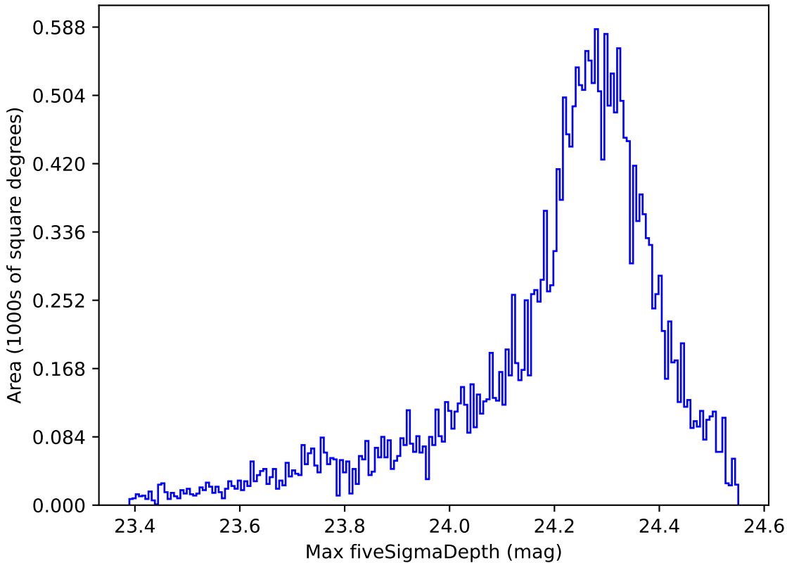
too_elab_r8_d3_gz_v3.4_10yrs All sky i band: Max fiveSigmaDepth
