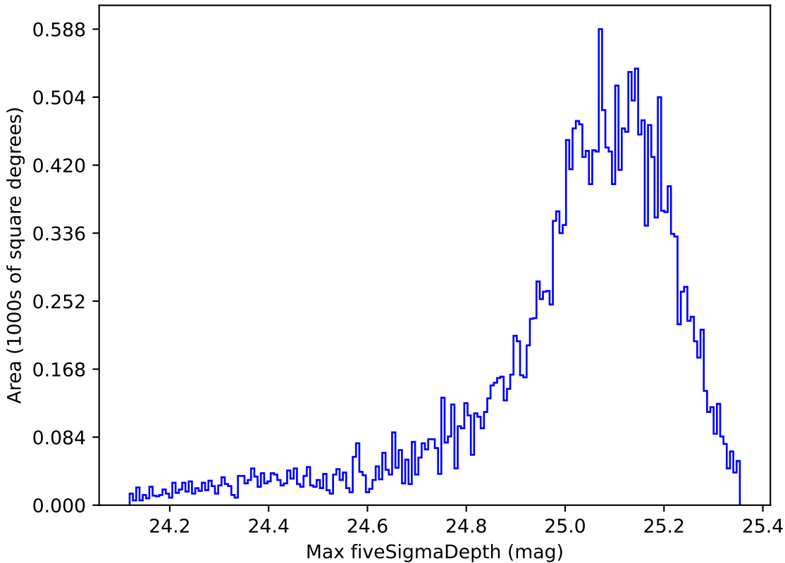
too_elab_r8_d3_gz_v3.4_10yrs All sky g band: Max fiveSigmaDepth
