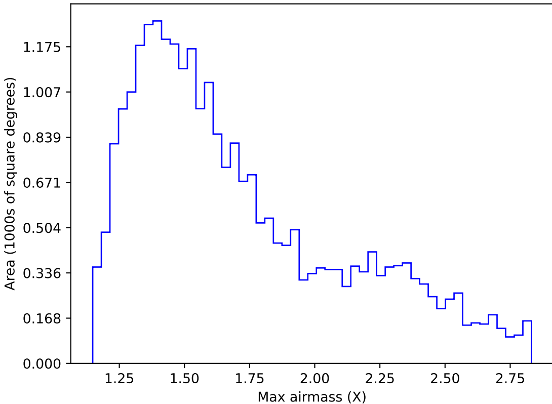
too_elab_r8_d3_gz_v3.4_10yrs Yr 1 z band: Max airmass
