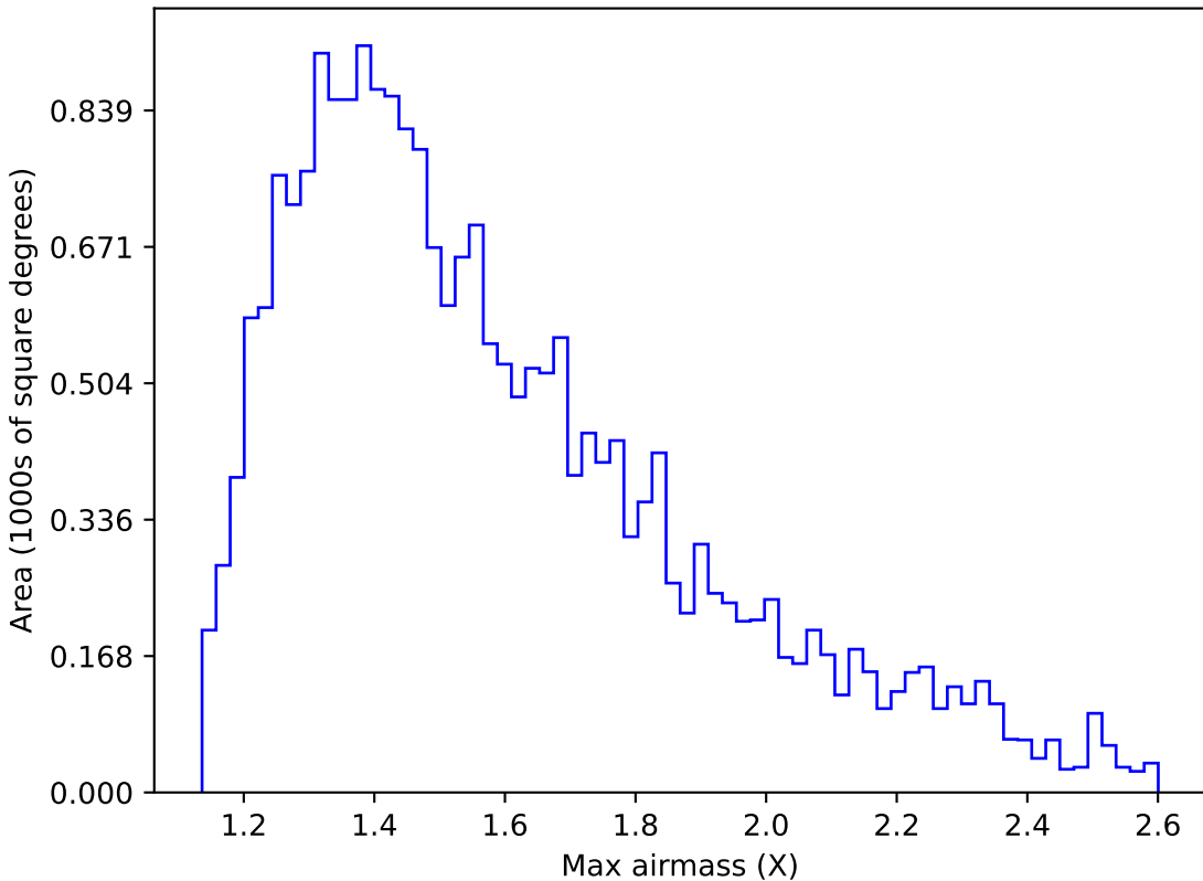
too_elab_r8_d3_gz_v3.4_10yrs Yr 1 y band: Max airmass
