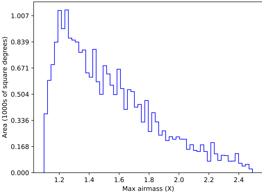
too_elab_r8_d3_gz_v3.4_10yrs Yr 1 u band: Max airmass
