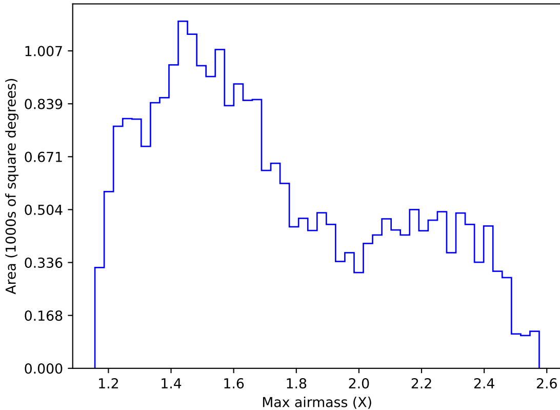
too_elab_r8_d3_gz_v3.4_10yrs Yr 1 r band: Max airmass
