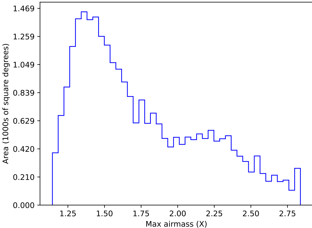
too_elab_r8_d3_gz_v3.4_10yrs Yr 1 i band: Max airmass
