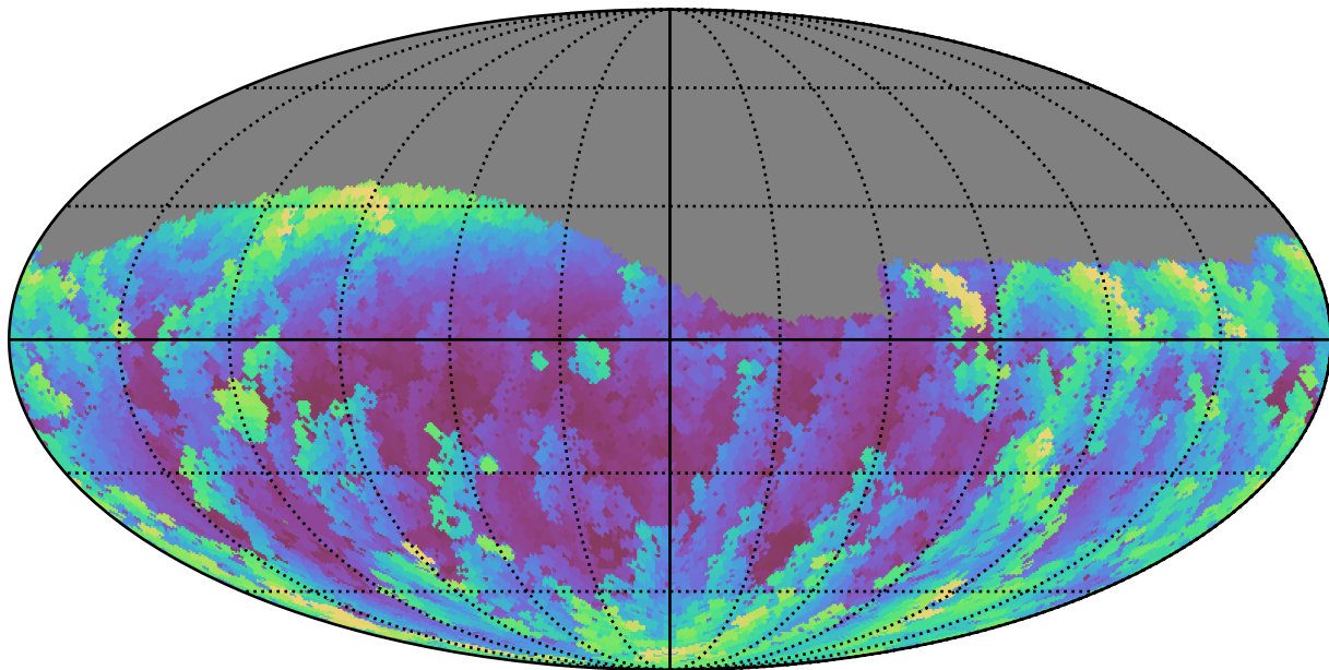
too_elab_r8_d3_gz_v3.4_10yrs Yr 1 g band: Max airmass
