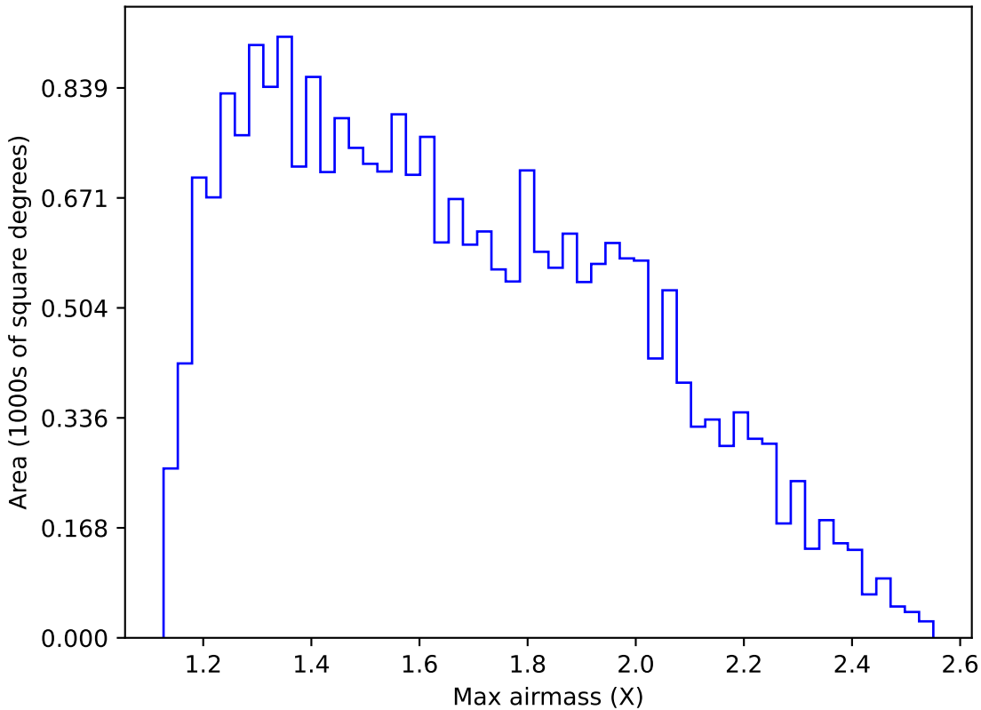
too_elab_r8_d3_gz_v3.4_10yrs Yr 1 g band: Max airmass
