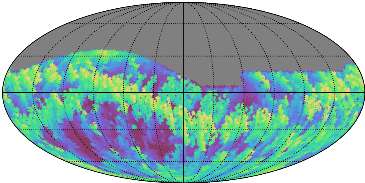
too_elab_r8_d3_gz_v3.4_10yrs Yr 1 all bands: Max airmass
