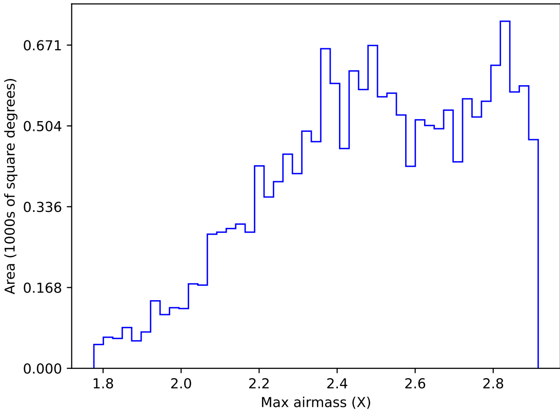
too_elab_r8_d3_gz_v3.4_10yrs WFD z band: Max airmass
