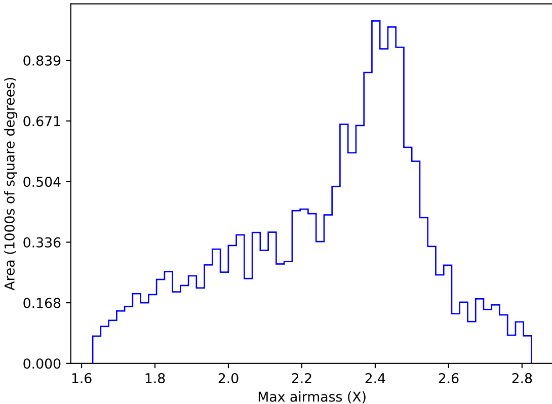
too_elab_r8_d3_gz_v3.4_10yrs WFD r band: Max airmass
