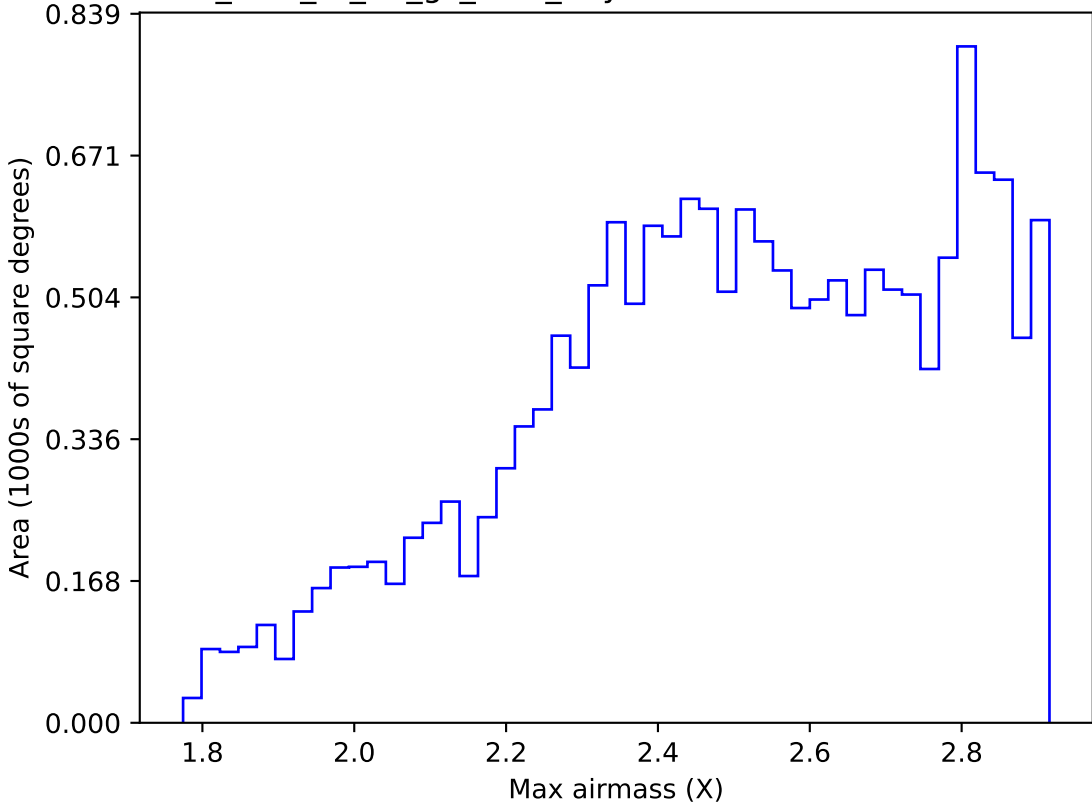
too_elab_r8_d3_gz_v3.4_10yrs WFD i band: Max airmass
