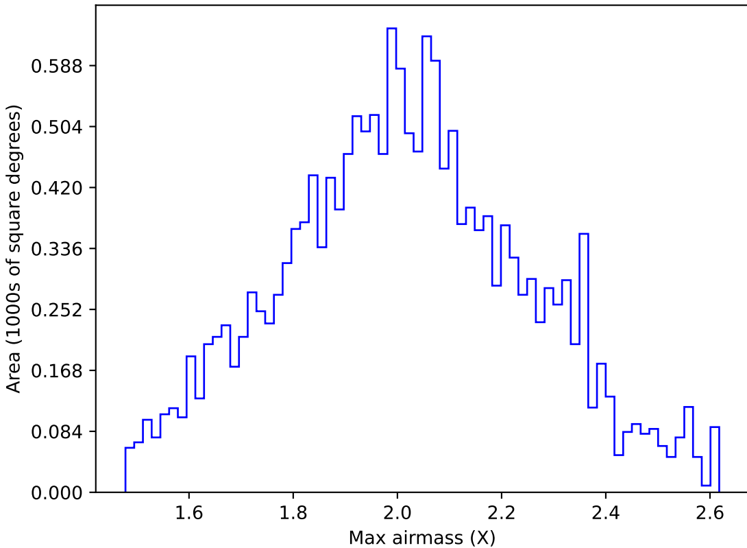
too_elab_r8_d3_gz_v3.4_10yrs WFD g band: Max airmass
