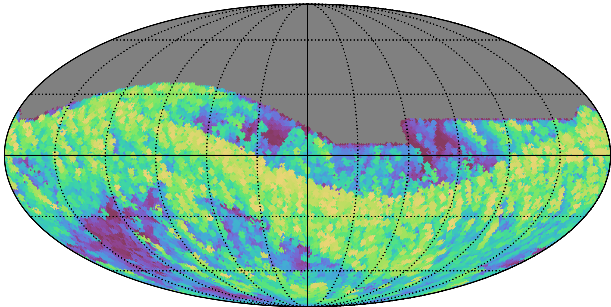
too_elab_r8_d3_gz_v3.4_10yrs All sky z band: Max airmass
