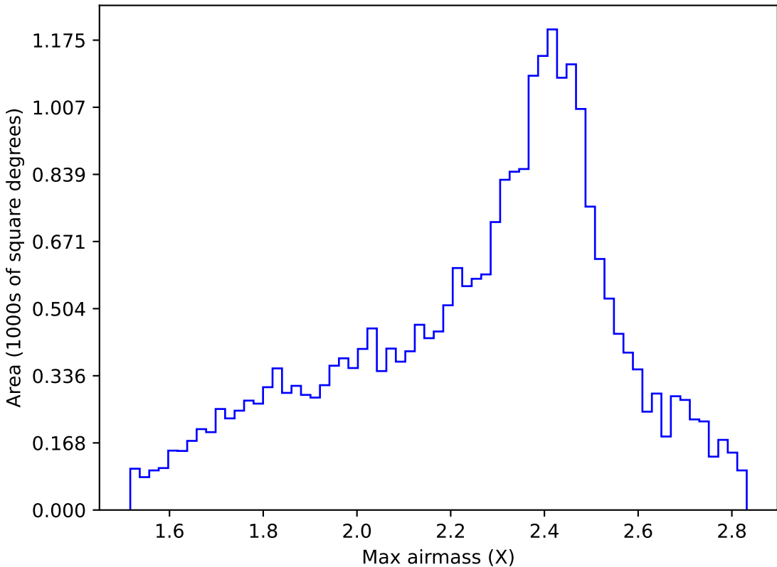
too_elab_r8_d3_gz_v3.4_10yrs All sky r band: Max airmass
