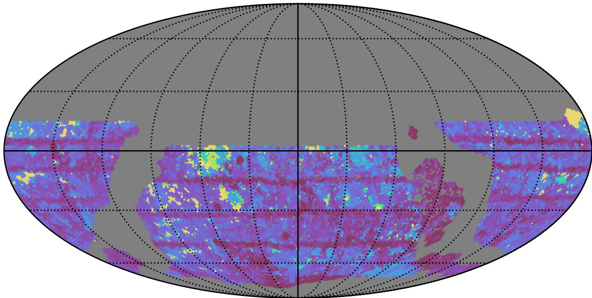
too_elab_r8_d3_gz_v3.4_10yrs WFD z band: Max Inter-Night Gap
