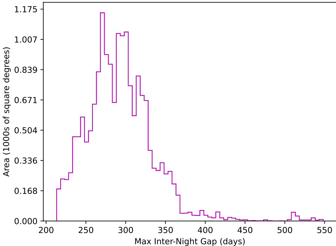
too_elab_r8_d3_gz_v3.4_10yrs WFD z band: Max Inter-Night Gap
