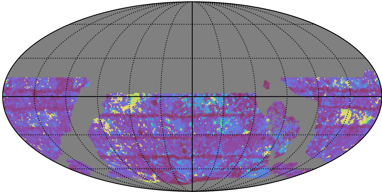
too_elab_r8_d3_gz_v3.4_10yrs WFD y band: Max Inter-Night Gap
