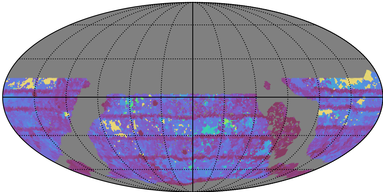
too_elab_r8_d3_gz_v3.4_10yrs WFD r band: Max Inter-Night Gap
