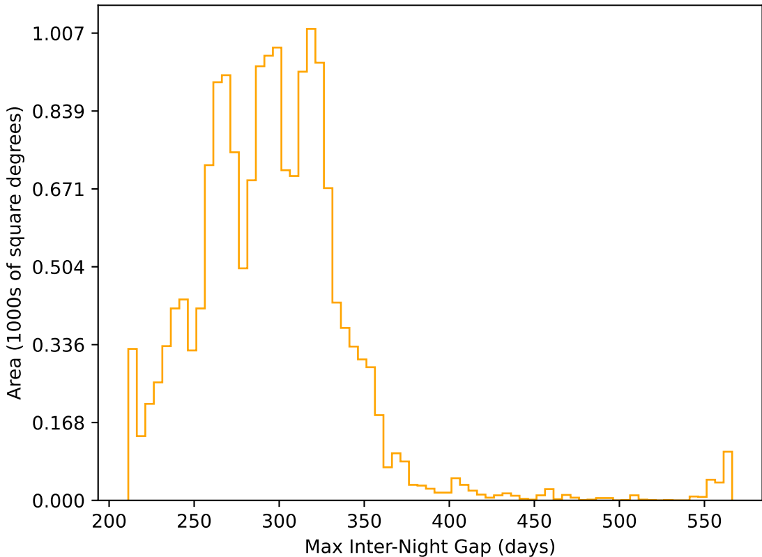
too_elab_r8_d3_gz_v3.4_10yrs WFD r band: Max Inter-Night Gap
