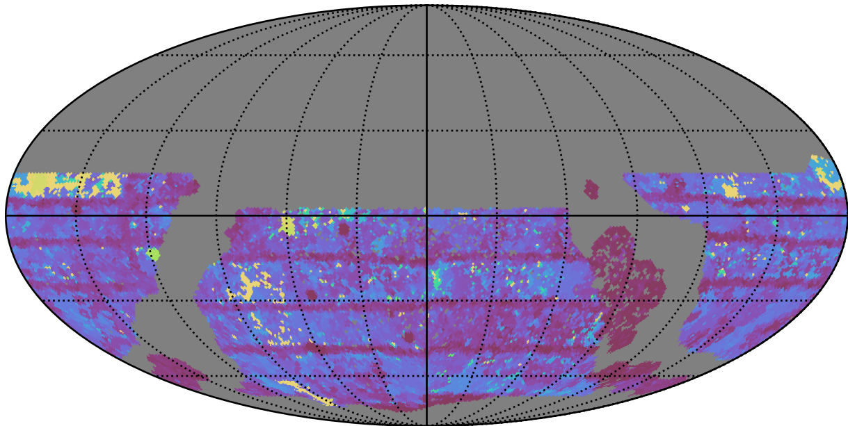
too_elab_r8_d3_gz_v3.4_10yrs WFD i band: Max Inter-Night Gap
