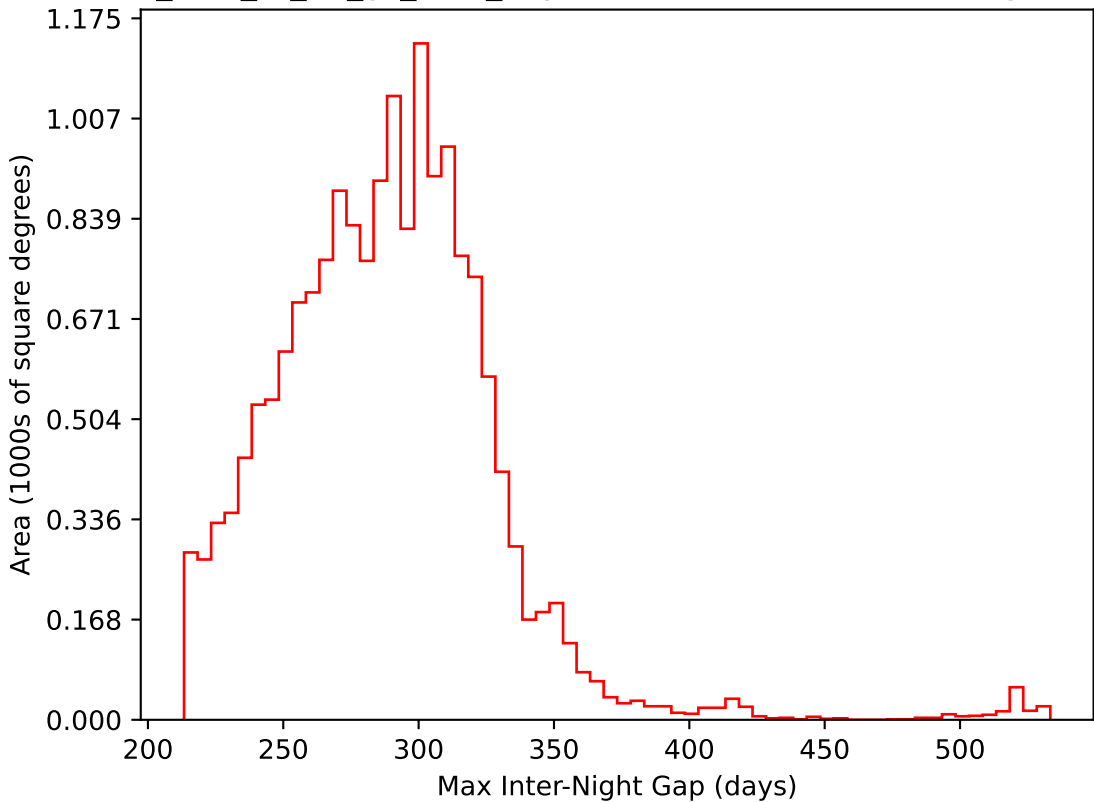
too_elab_r8_d3_gz_v3.4_10yrs WFD i band: Max Inter-Night Gap
