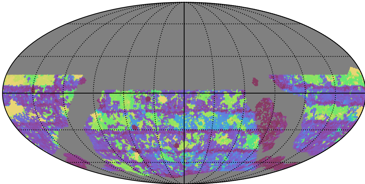
too_elab_r8_d3_gz_v3.4_10yrs WFD g band: Max Inter-Night Gap
