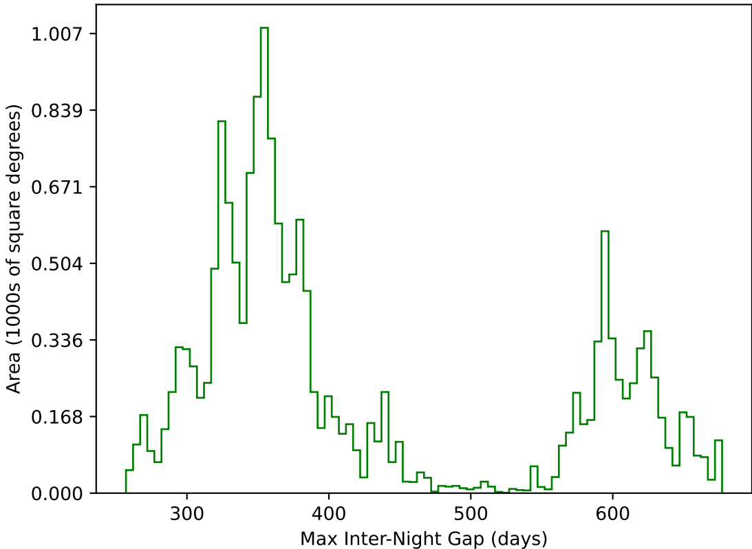
too_elab_r8_d3_gz_v3.4_10yrs WFD g band: Max Inter-Night Gap
