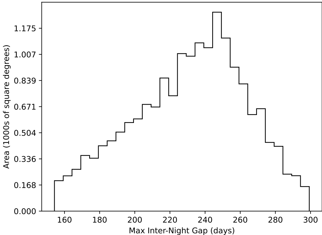
too_elab_r8_d3_gz_v3.4_10yrs WFD all bands: Max Inter-Night Gap
