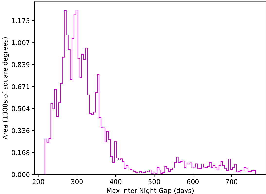
too_elab_r8_d3_gz_v3.4_10yrs All sky z band: Max Inter-Night Gap
