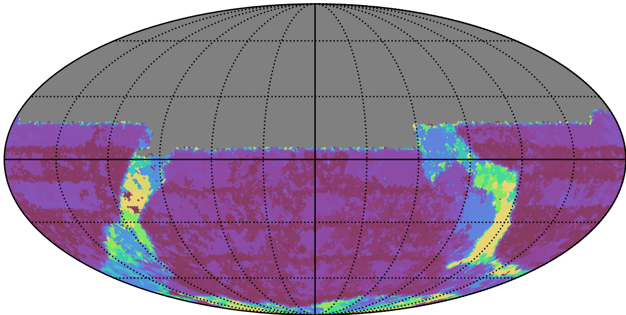
too_elab_r8_d3_gz_v3.4_10yrs All sky u band: Max Inter-Night Gap
