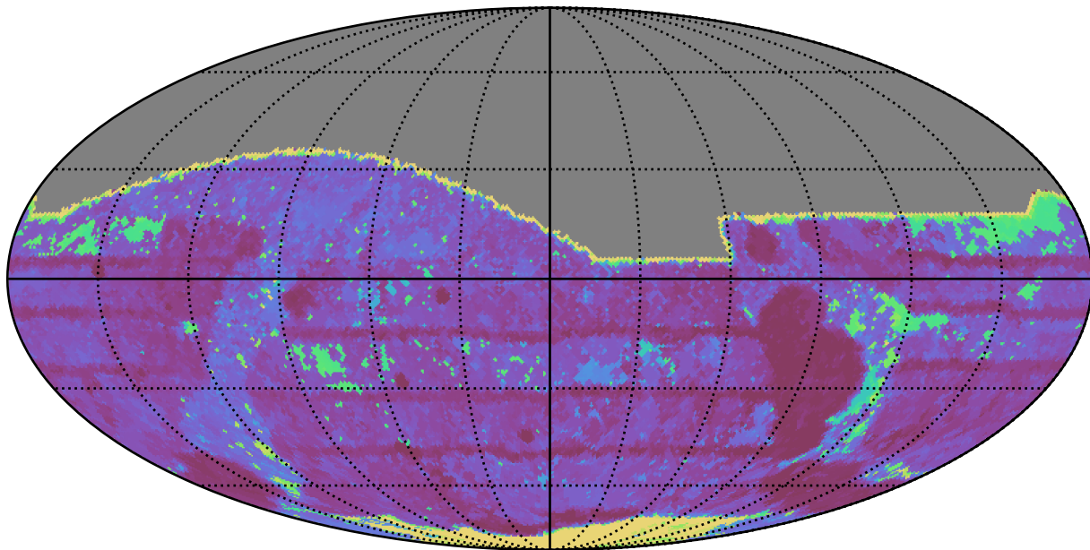
too_elab_r8_d3_gz_v3.4_10yrs All sky r band: Max Inter-Night Gap
