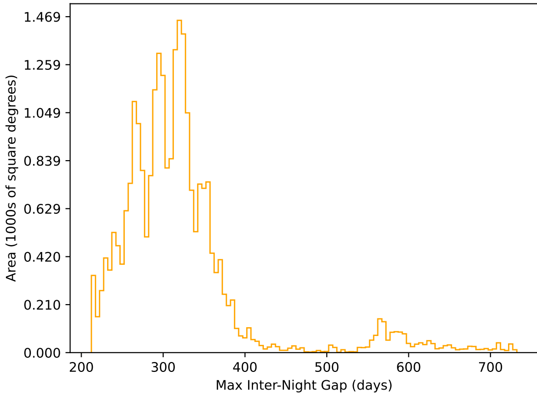
too_elab_r8_d3_gz_v3.4_10yrs All sky r band: Max Inter-Night Gap
