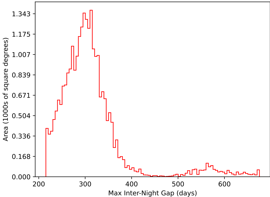
too_elab_r8_d3_gz_v3.4_10yrs All sky i band: Max Inter-Night Gap
