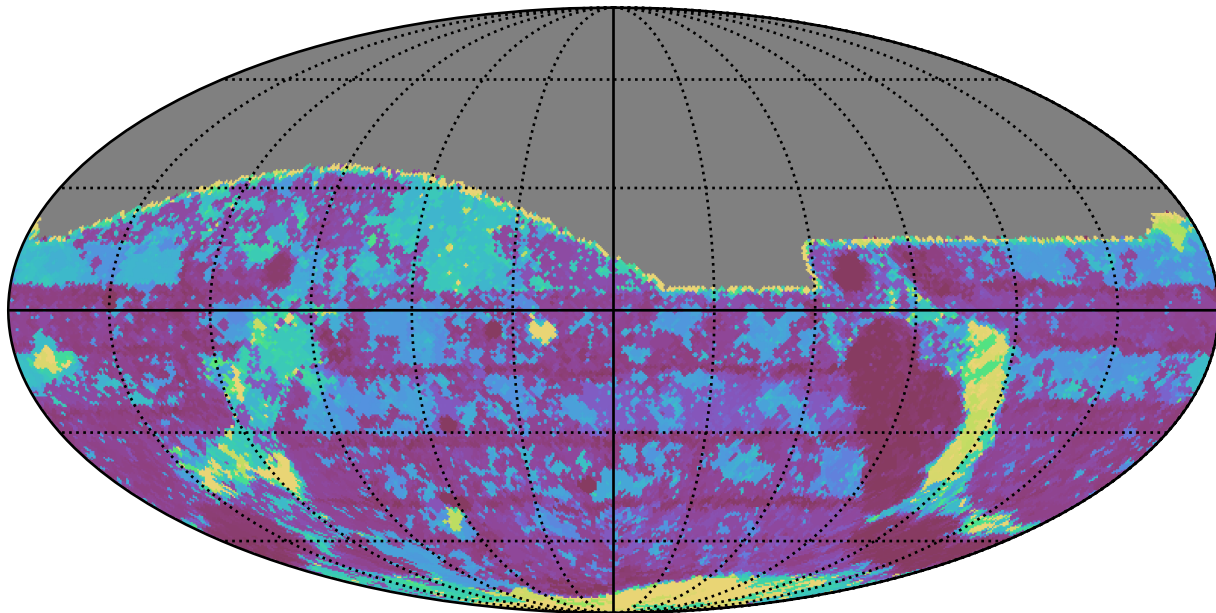
too_elab_r8_d3_gz_v3.4_10yrs All sky g band: Max Inter-Night Gap
