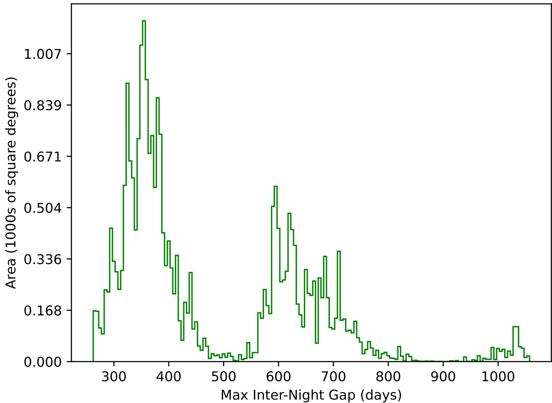
too_elab_r8_d3_gz_v3.4_10yrs All sky g band: Max Inter-Night Gap
