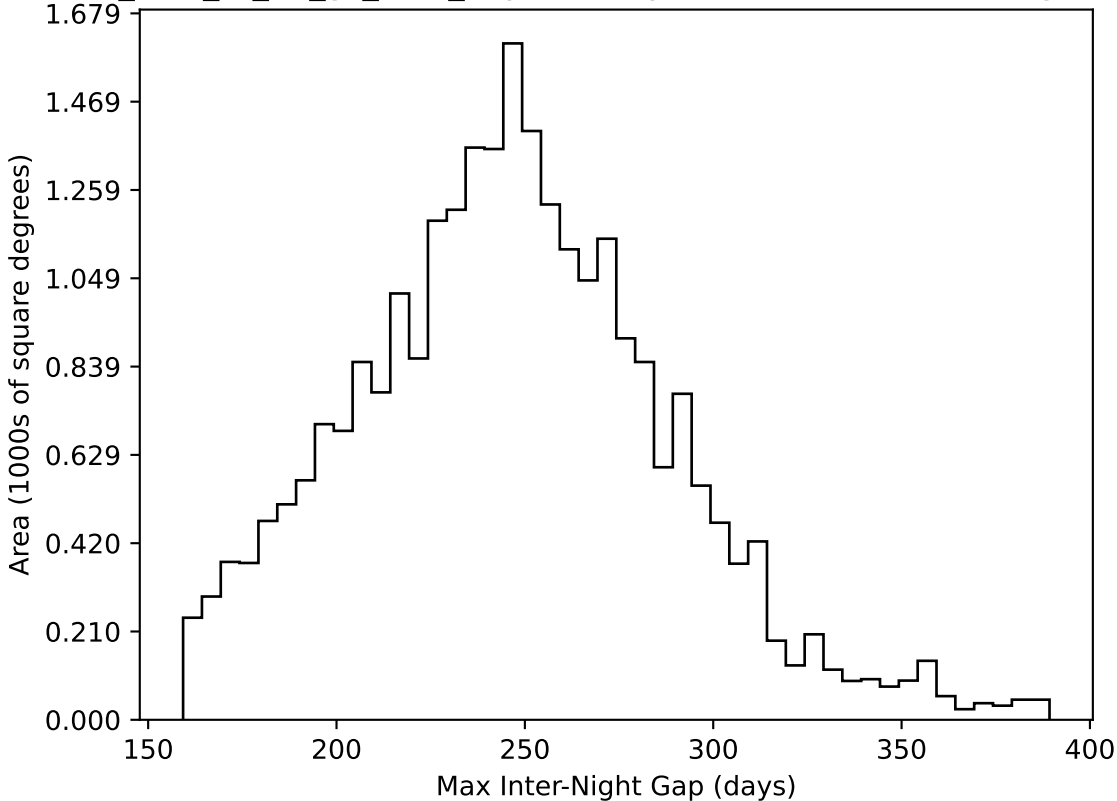
too_elab_r8_d3_gz_v3.4_10yrs All sky all bands: Max Inter-Night Gap
