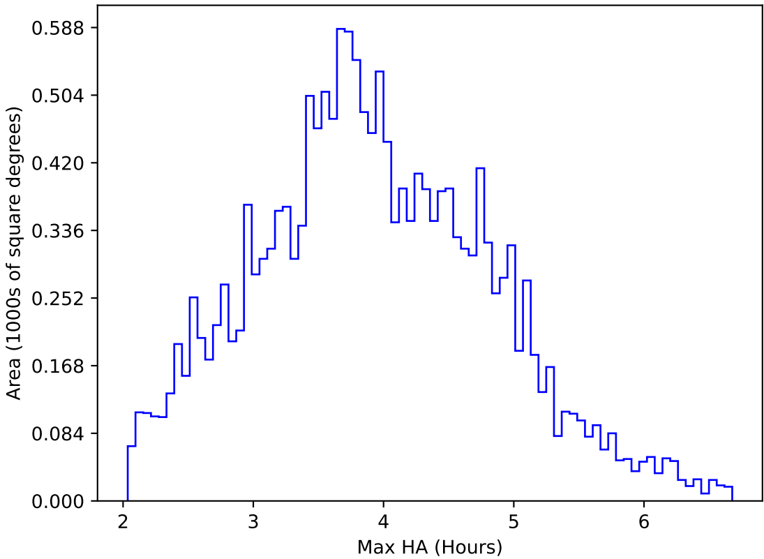
too_elab_r8_d3_gz_v3.4_10yrs WFD u band: Max HA
