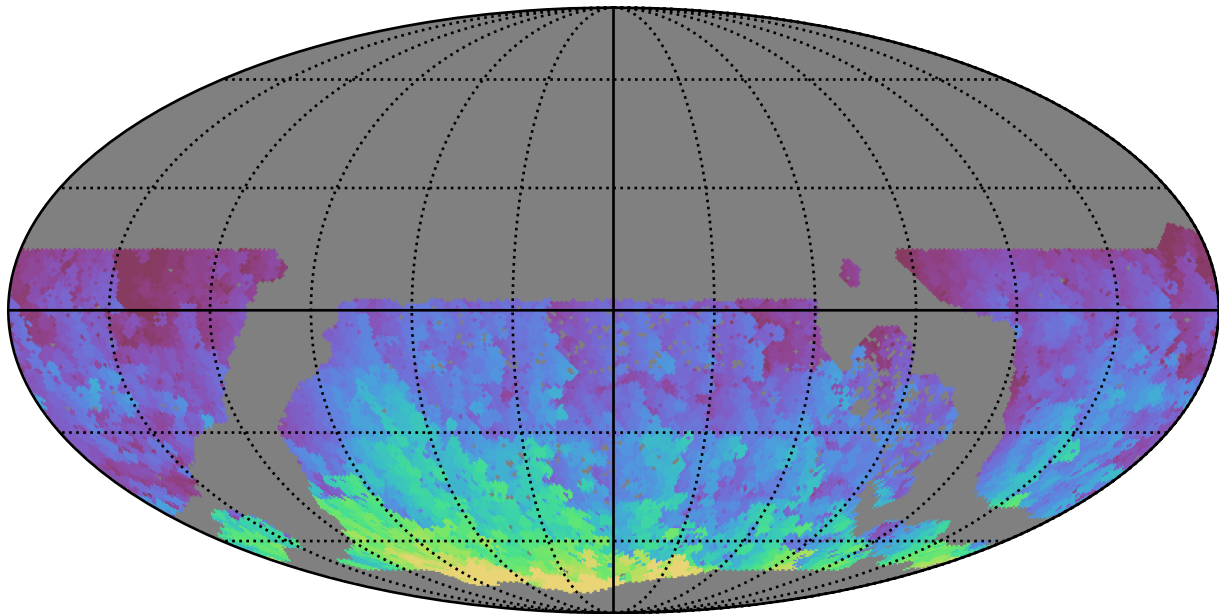
too_elab_r8_d3_gz_v3.4_10yrs WFD r band: Max HA
