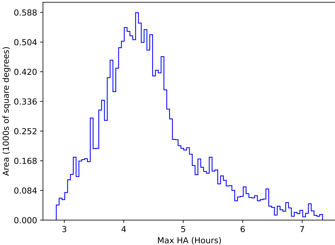
too_elab_r8_d3_gz_v3.4_10yrs WFD r band: Max HA
