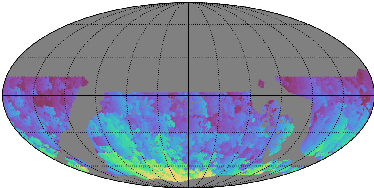
too_elab_r8_d3_gz_v3.4_10yrs WFD g band: Max HA
