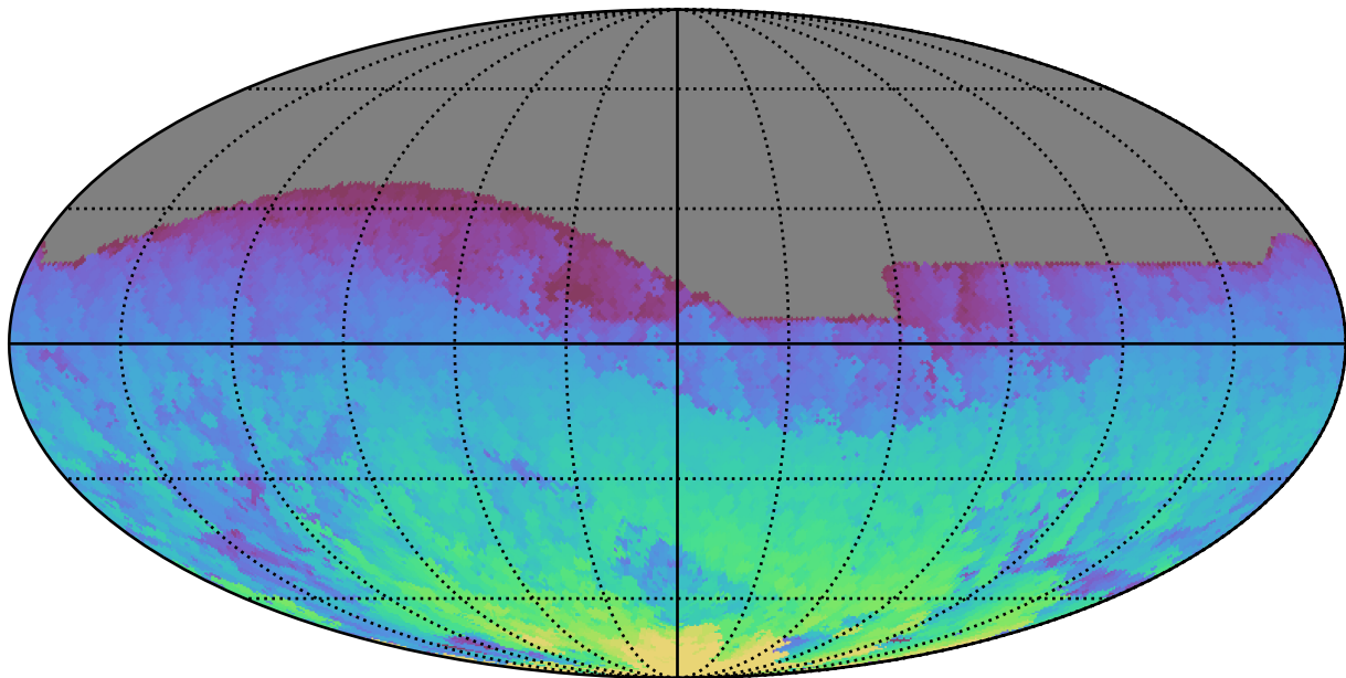
too_elab_r8_d3_gz_v3.4_10yrs All sky z band: Max HA
