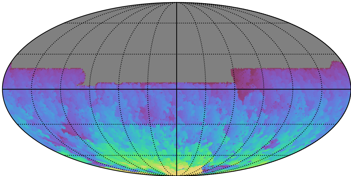
too_elab_r8_d3_gz_v3.4_10yrs All sky y band: Max HA
