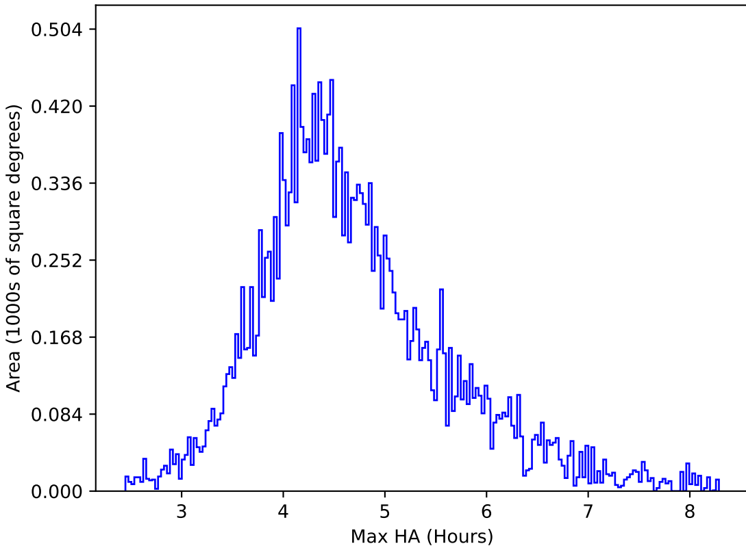
too_elab_r8_d3_gz_v3.4_10yrs All sky y band: Max HA
