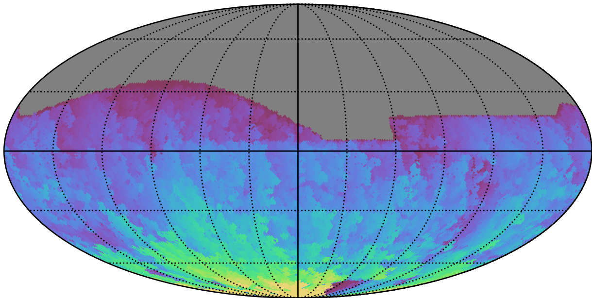
too_elab_r8_d3_gz_v3.4_10yrs All sky r band: Max HA
