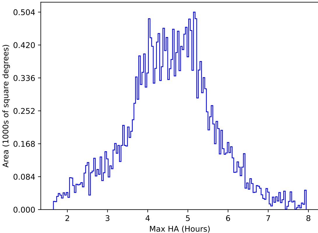
too_elab_r8_d3_gz_v3.4_10yrs All sky i band: Max HA
