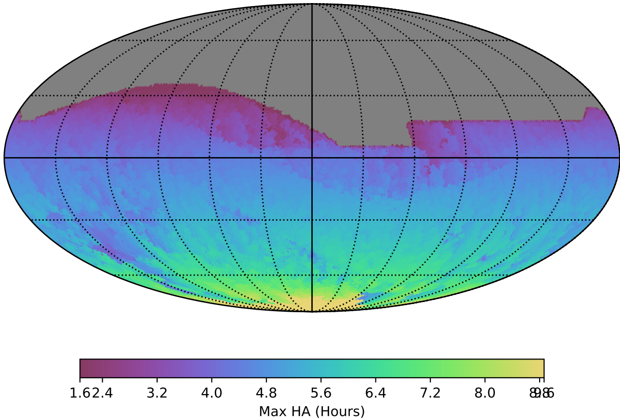
too_elab_r8_d3_gz_v3.4_10yrs All sky all bands: Max HA
