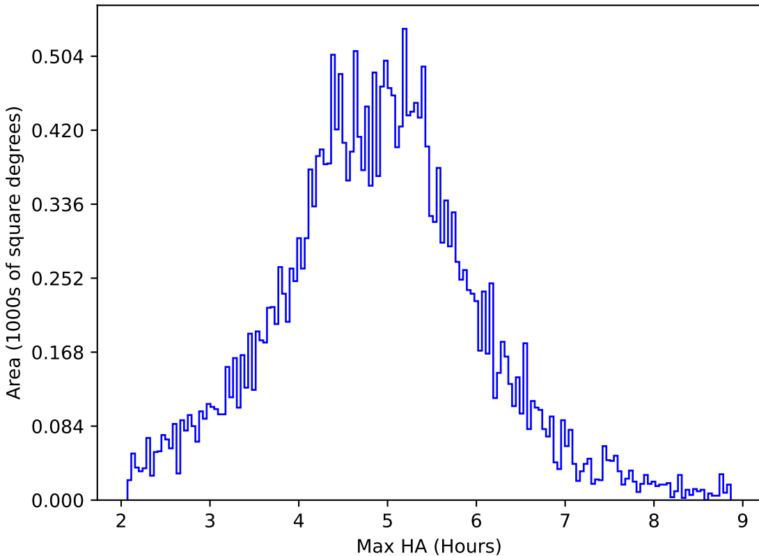
too_elab_r8_d3_gz_v3.4_10yrs All sky all bands: Max HA
