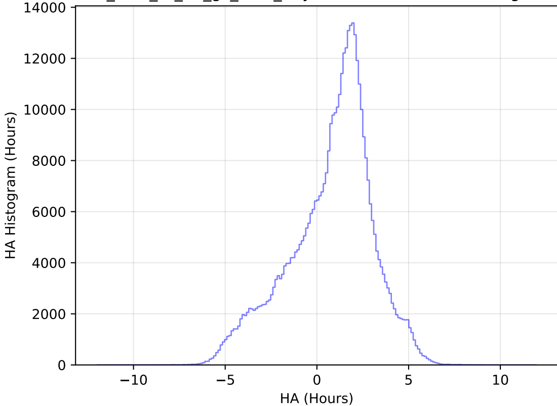
too_elab_r8_d3_gz_v3.4_10yrs WFD z band: HA Histogram
