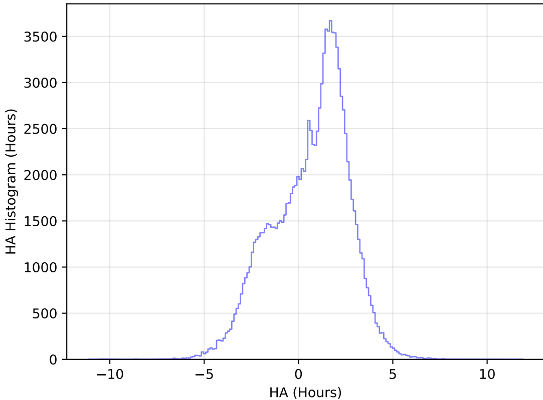
too_elab_r8_d3_gz_v3.4_10yrs WFD u band: HA Histogram
