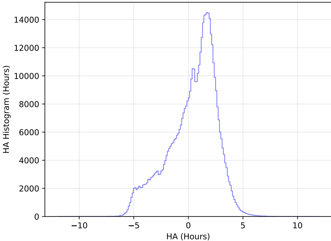
too_elab_r8_d3_gz_v3.4_10yrs WFD r band: HA Histogram
