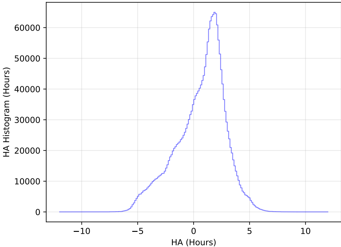
too_elab_r8_d3_gz_v3.4_10yrs WFD all bands: HA Histogram
